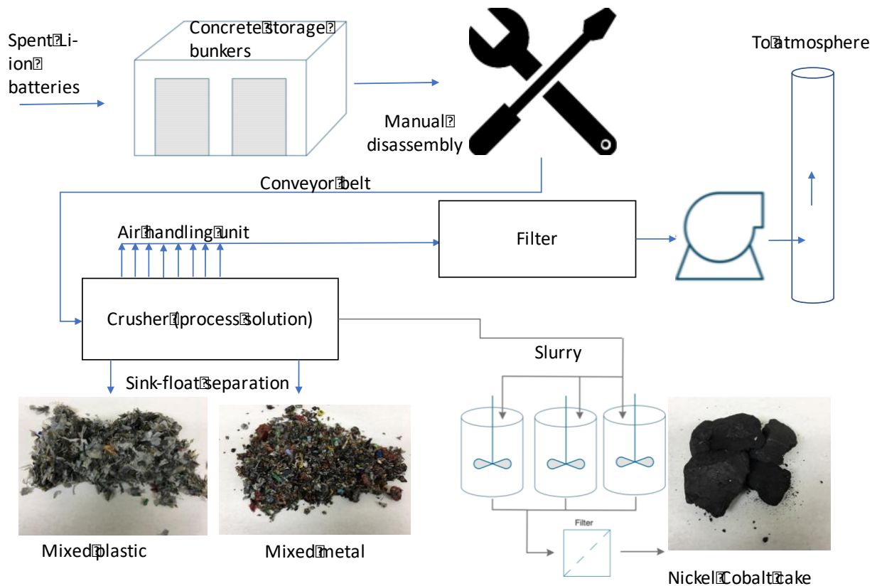
Figure 3 Retrieve Technology's recycling process flow.
